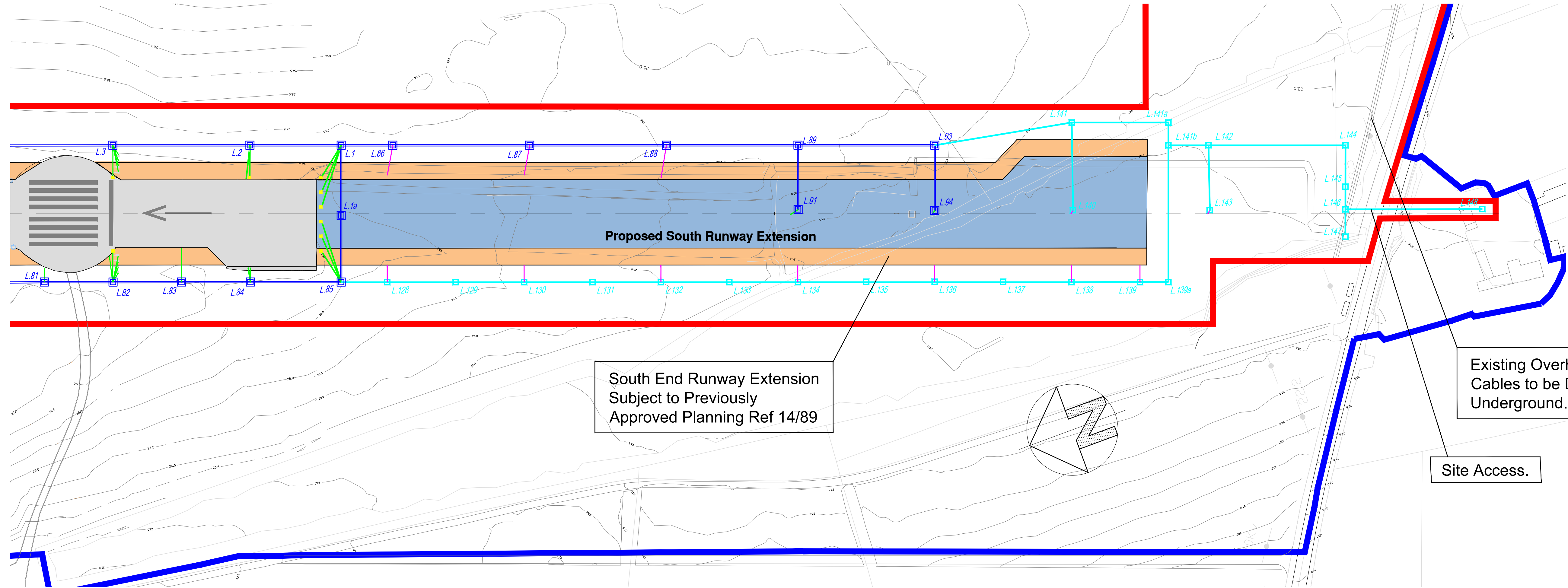
SOUTH END RUNWAY EXTENSION LIGHTING LAYOUT
